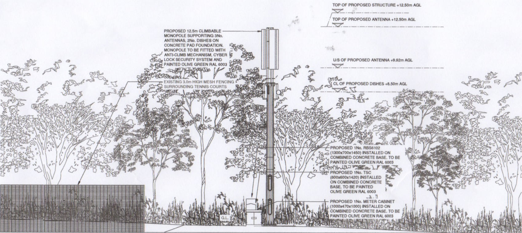
PROPOSED SITE ELEVATION (SCALE 1:100)
